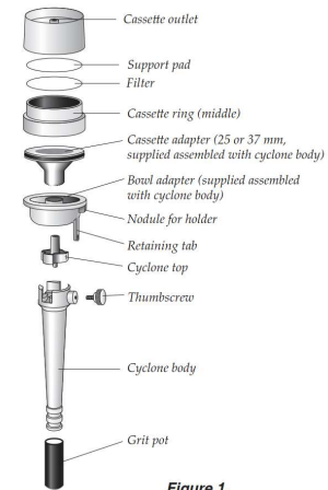
Figure 1. GS-3 Cyclone with filter cassette — exploded view
